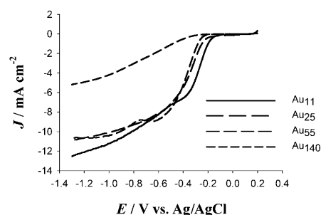
Figure 4. RDE voltammograms of varied Au_x/GC electrodes in 0.1 M KOH aqueous solution saturated by oxygen. Experimental conditions were the same as in Figure 3. Rotation rate 3600 rpm.
